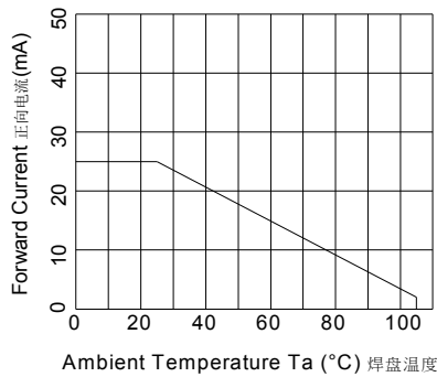
Ambient Temperature VS. Forward Current Ta-IF曲线
