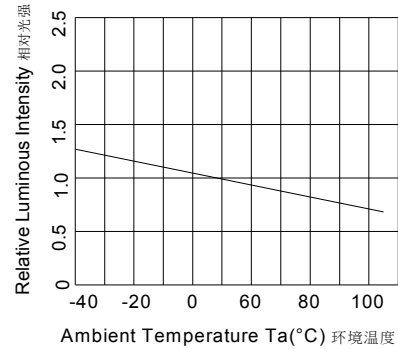
Ambient Temperature VS. Relative Intensity Ta-IV曲线
