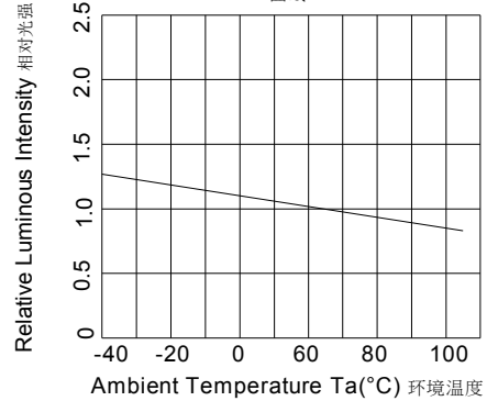
Ambient Temperature VS. Relative Intensity Ta-IV曲线
