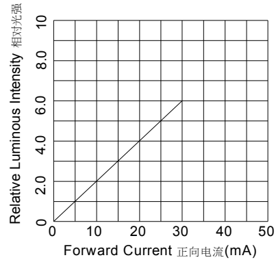
Forward Current VS. Relative Intensity IF-IV曲线
