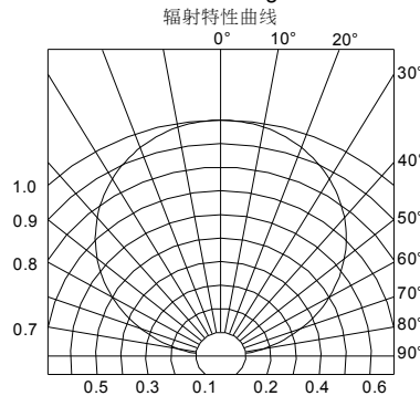
Radiation Diagram
