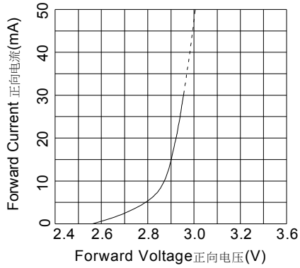
Volt-Ampere Characteristics VF-IF曲线
