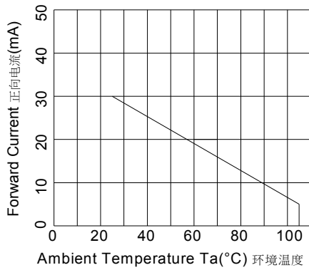
Ambient Temperature VS. Forward Current Ta-IF曲线
